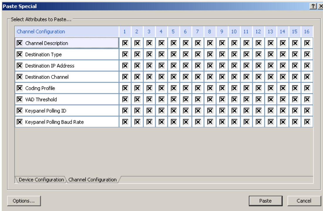
FIGURE 27. Channel Configuration Page - Paste Special Window
