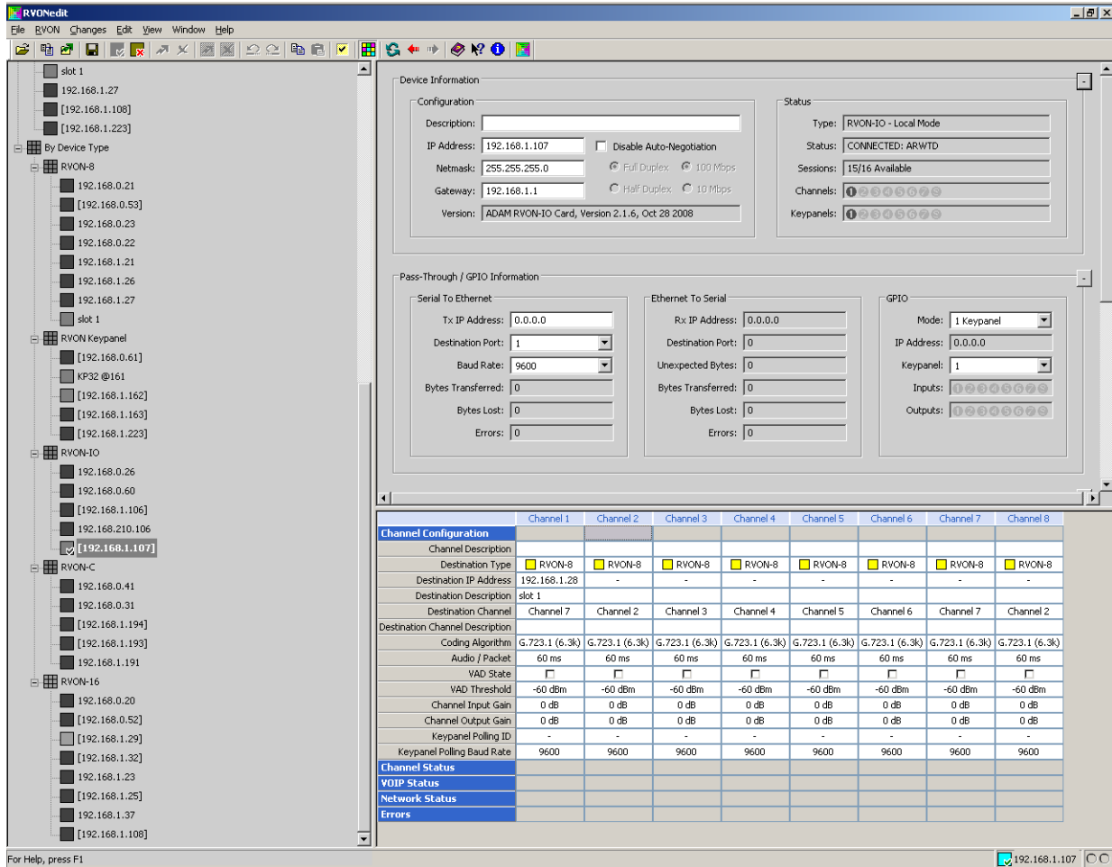
FIGURE 10. Channel Configuration and Status
