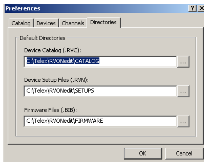
FIGURE 22. Directories Page - Preferences Window
