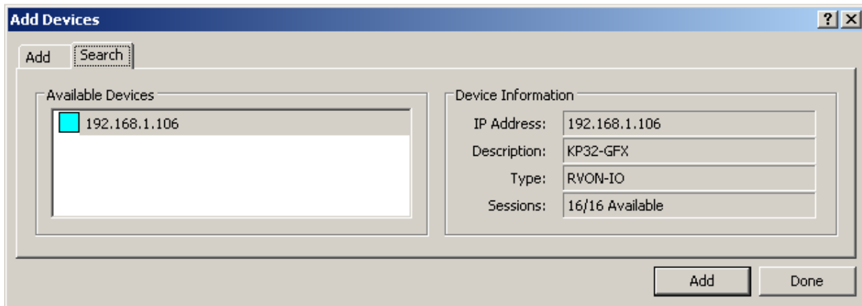
FIGURE 24. Search Page - Add Devices Window
