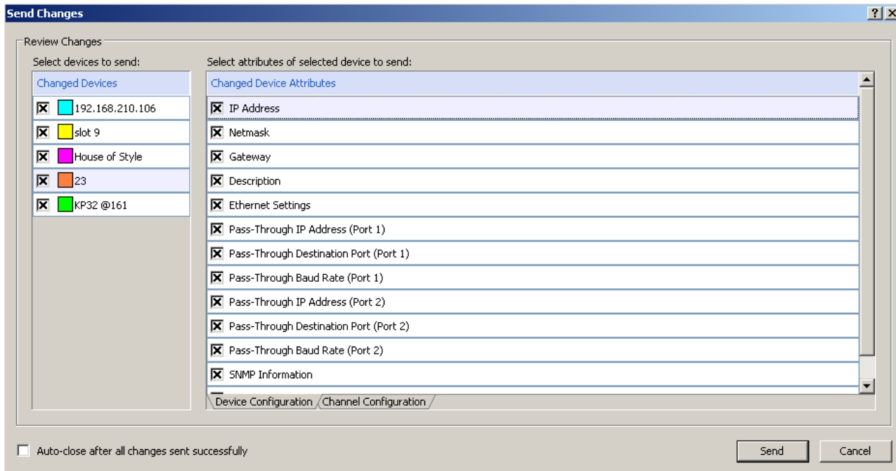
FIGURE 26. Device Configuration Page - Send Changes Window
