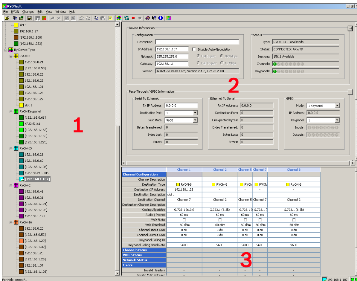
FIGURE 2. RVONedit Main Application Window
