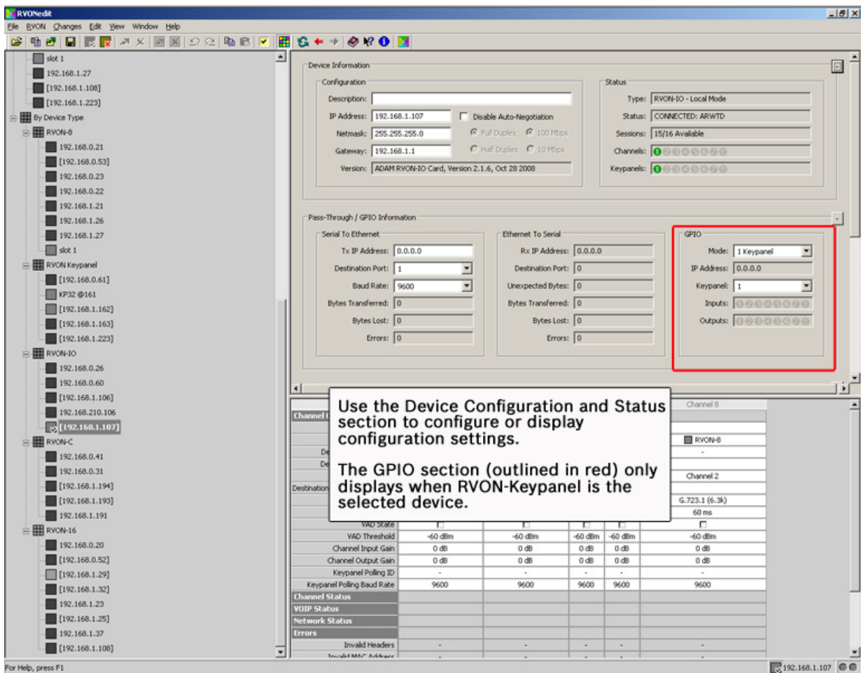
FIGURE 4. Device Configuration and Status Section
