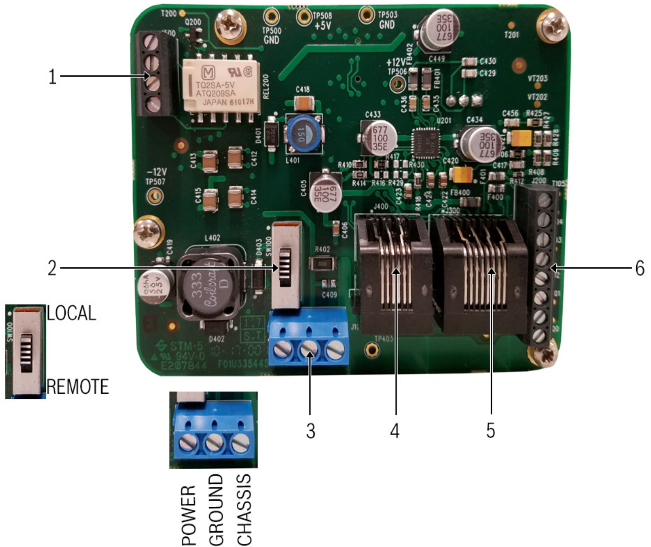
FIGURE 7. Connections Board of the WKP-1.
