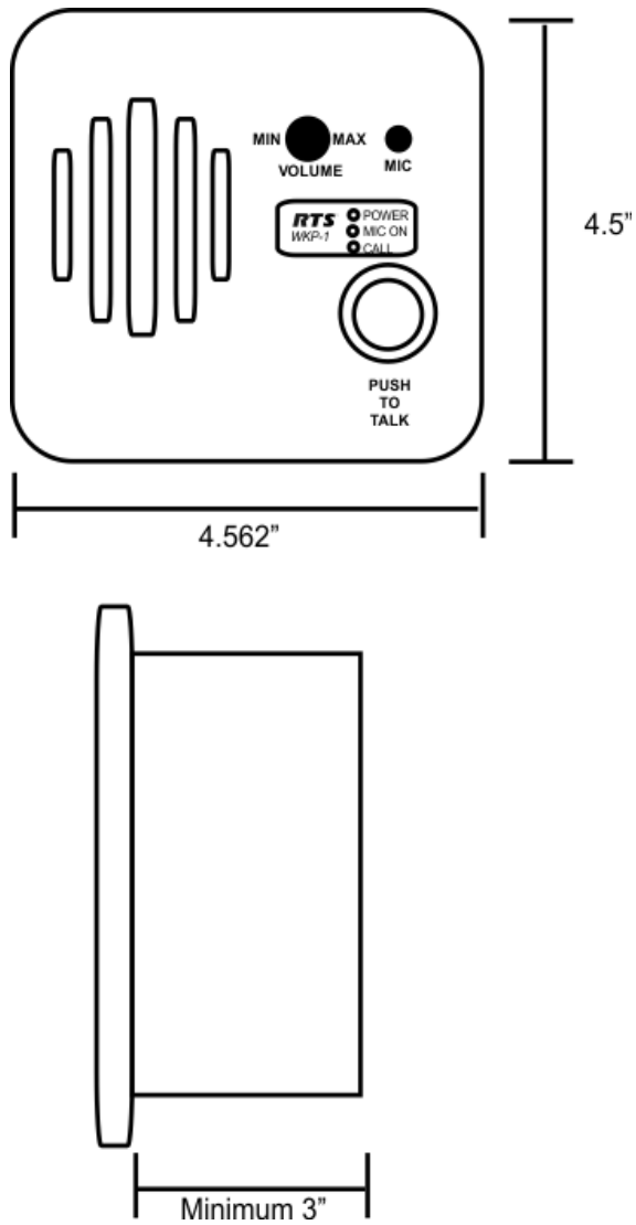
FIGURE 2. WKP-1 Industrial Keypanel size requirements
