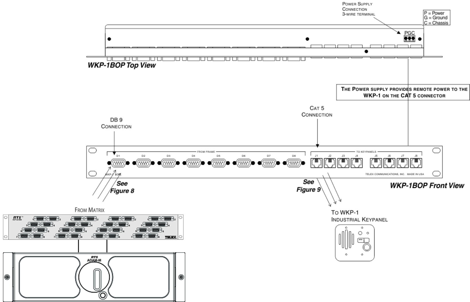
FIGURE 10. WKP-1 BOP System Diagram
